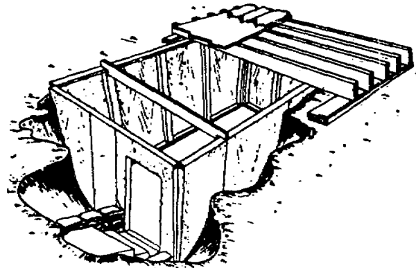
Figure 1-59. Air-transportable underground assault bunker (prefab).
